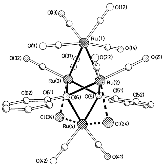
Figure 4. The structure of compound (13) in the crystal (radii arbitrary, H atoms omitted). The interactions Ru(2) \cdots Ru(3) , Ru(2) \cdots Ru(4) , and Ru(3) \cdots Ru(4) are all > 3.1 \text{ \AA} and are not regarded as bonds (see text)
